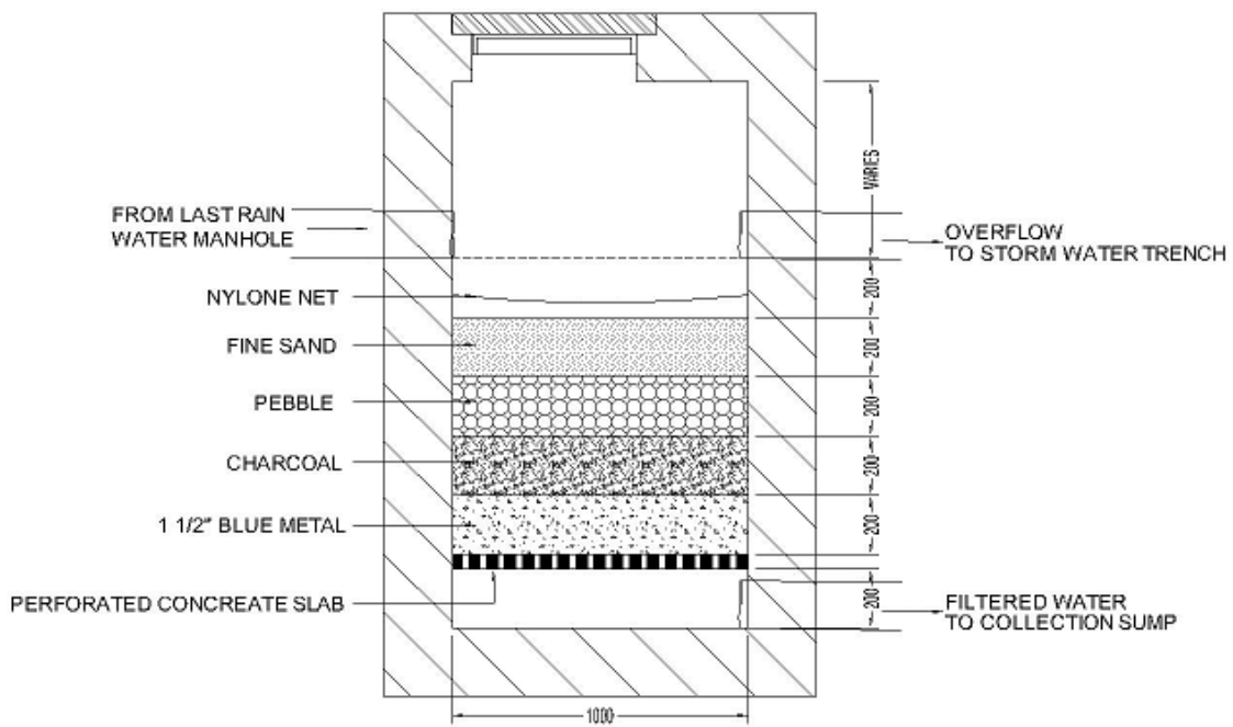
RAIN WATER FILTER DETAIL
